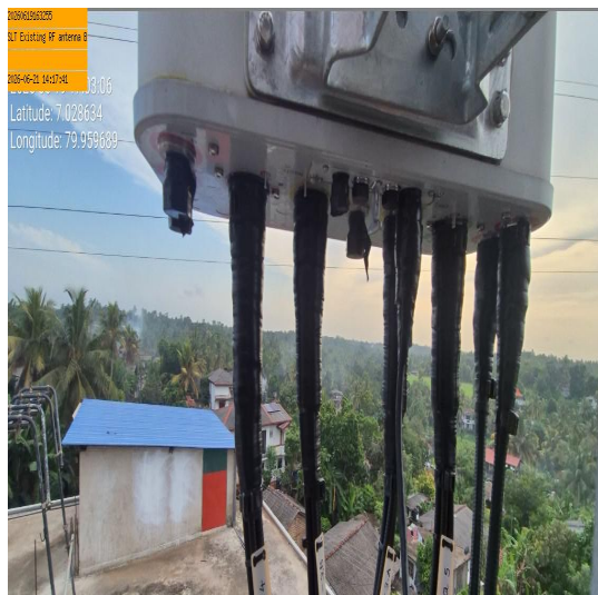
SLT Existing RF antenna Bottom View sector 03
