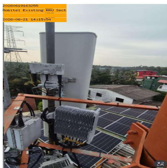
Mobitel Existing RRU Sector 01 image2
