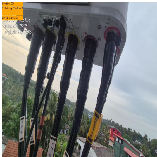
SLT Existing RF antenna Bottom View sector 01
