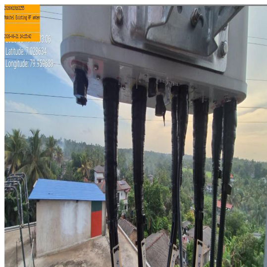
Mobitel Existing RF antenna Bottom View sector 03
