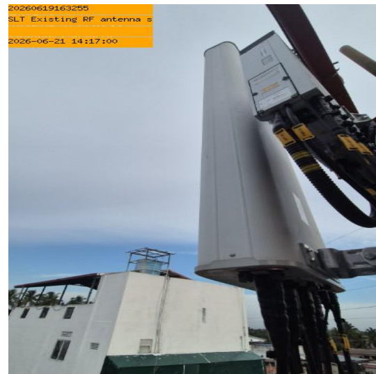
SLT Existing RF antenna sector 02
