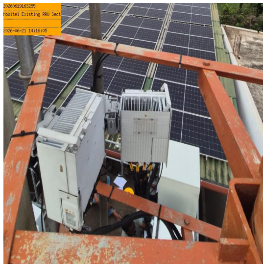
Mobitel Existing RRU Sector 02 image2
