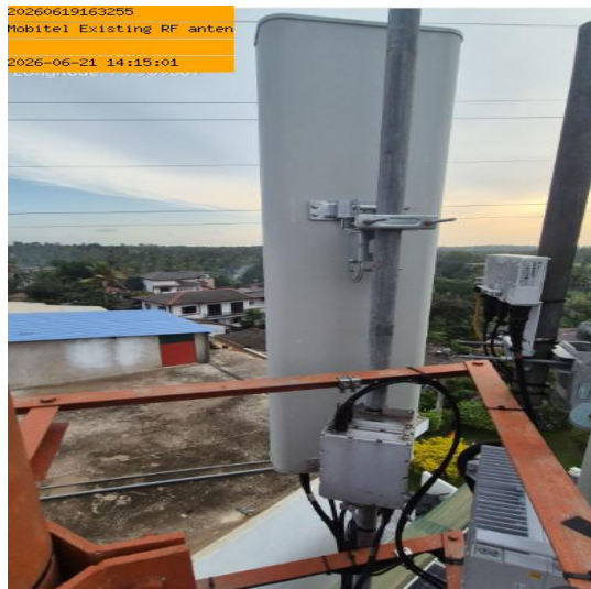
Mobitel Existing RF antenna sector 03
