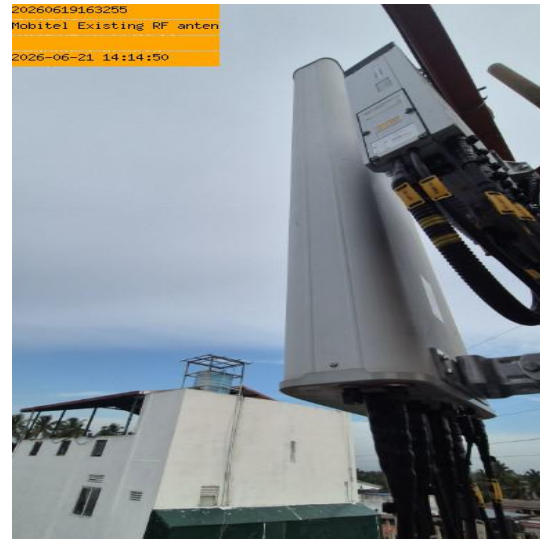
Mobitel Existing RF antenna sector 02
